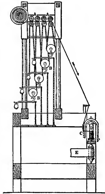
FIG. 1. THE THROSTLE
